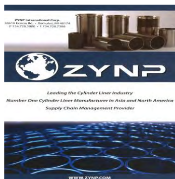
Company brochure
